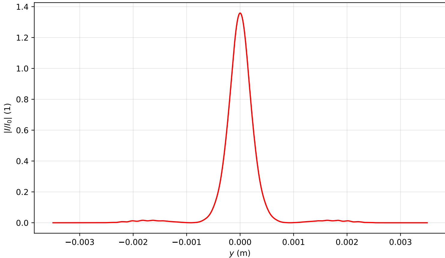
Intensity profile I(x=0, y, z=1.274)/I_0 , \text{Pin}=1.0\text{Pcr} , artificial time
